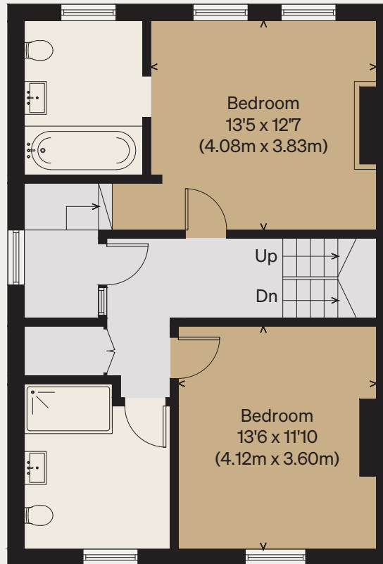
SECOND FLOOR
