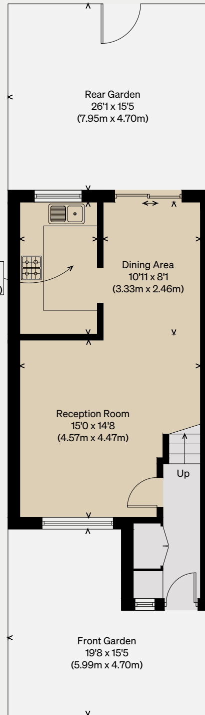
GROUND FLOOR
