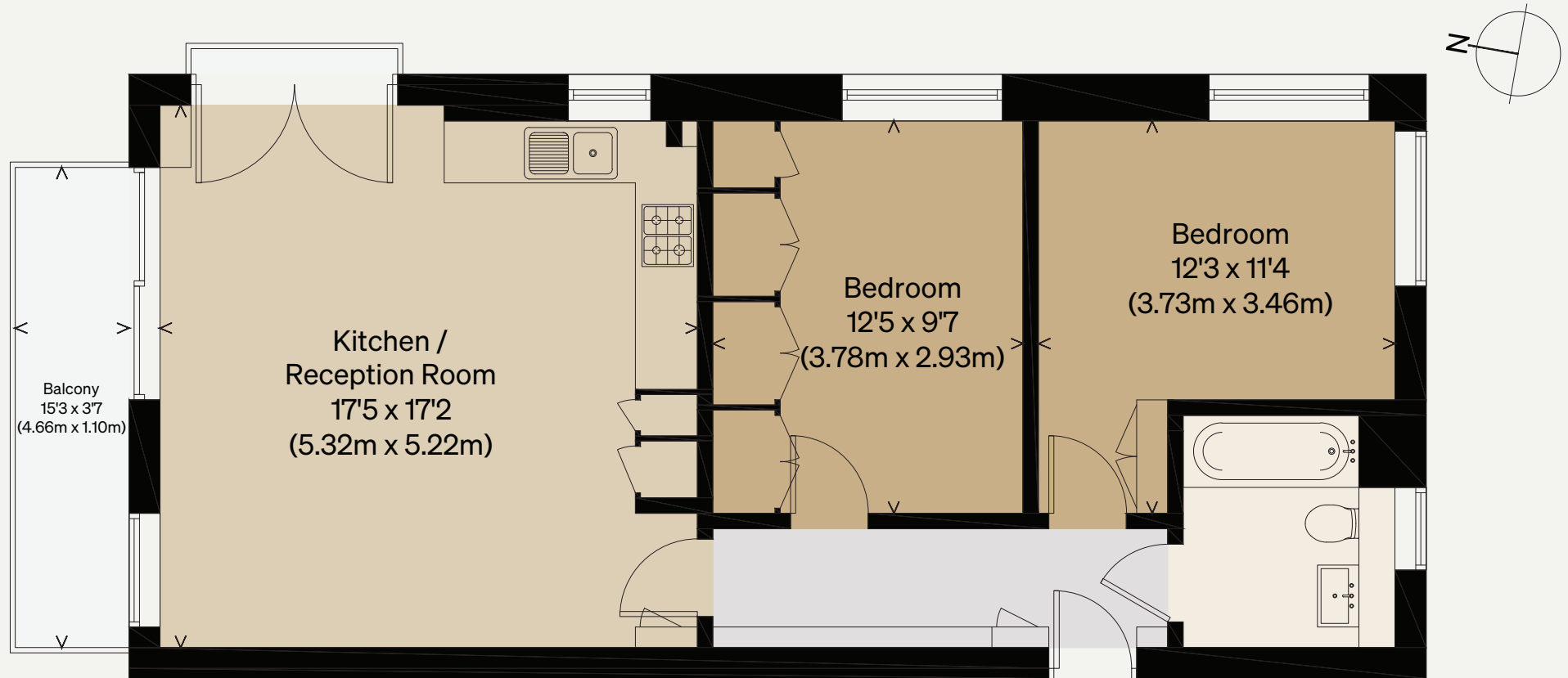
FOURTH FLOOR
