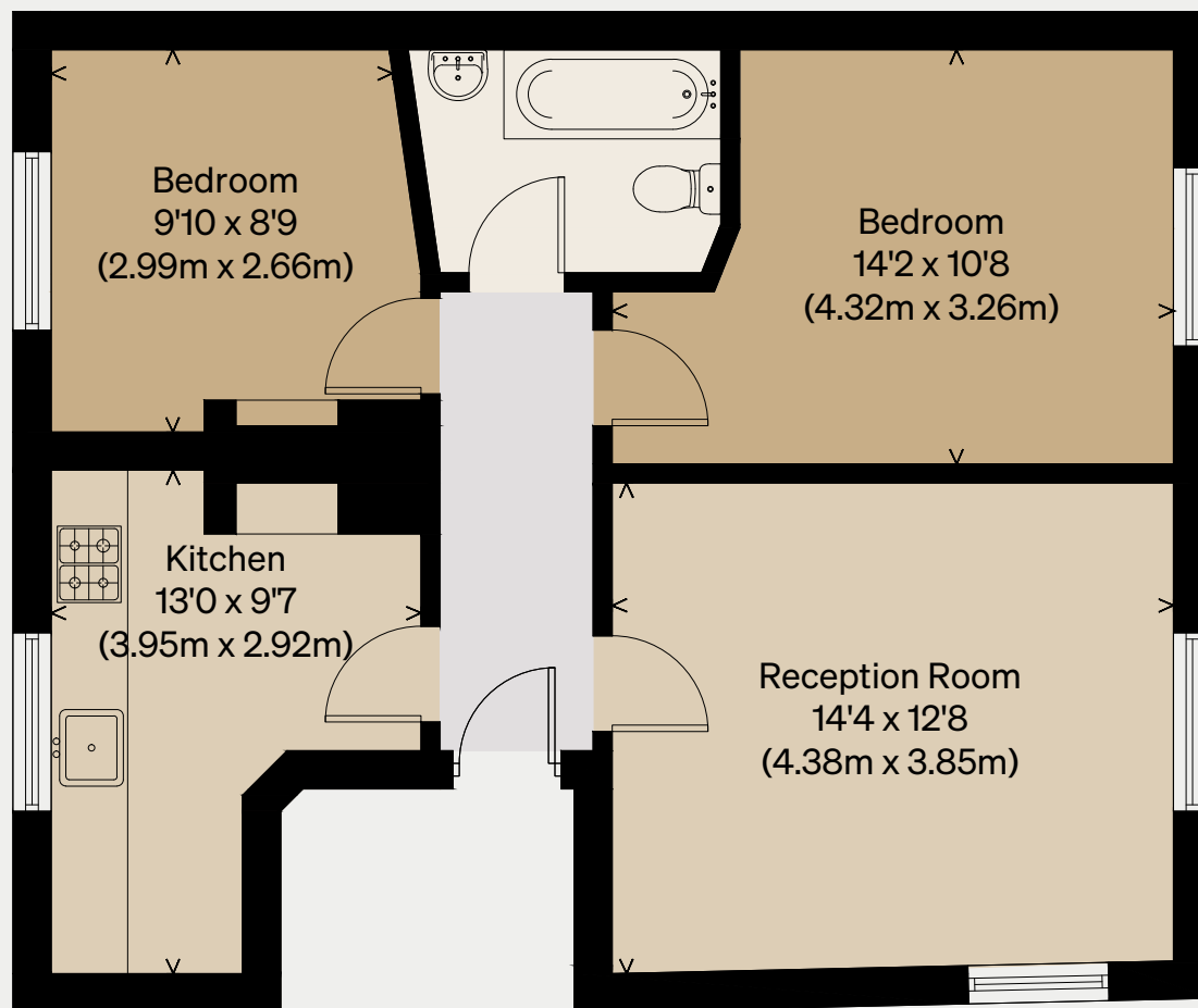
FIRST FLOOR
