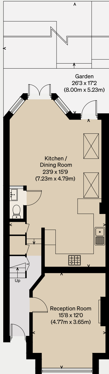
GROUND FLOOR
