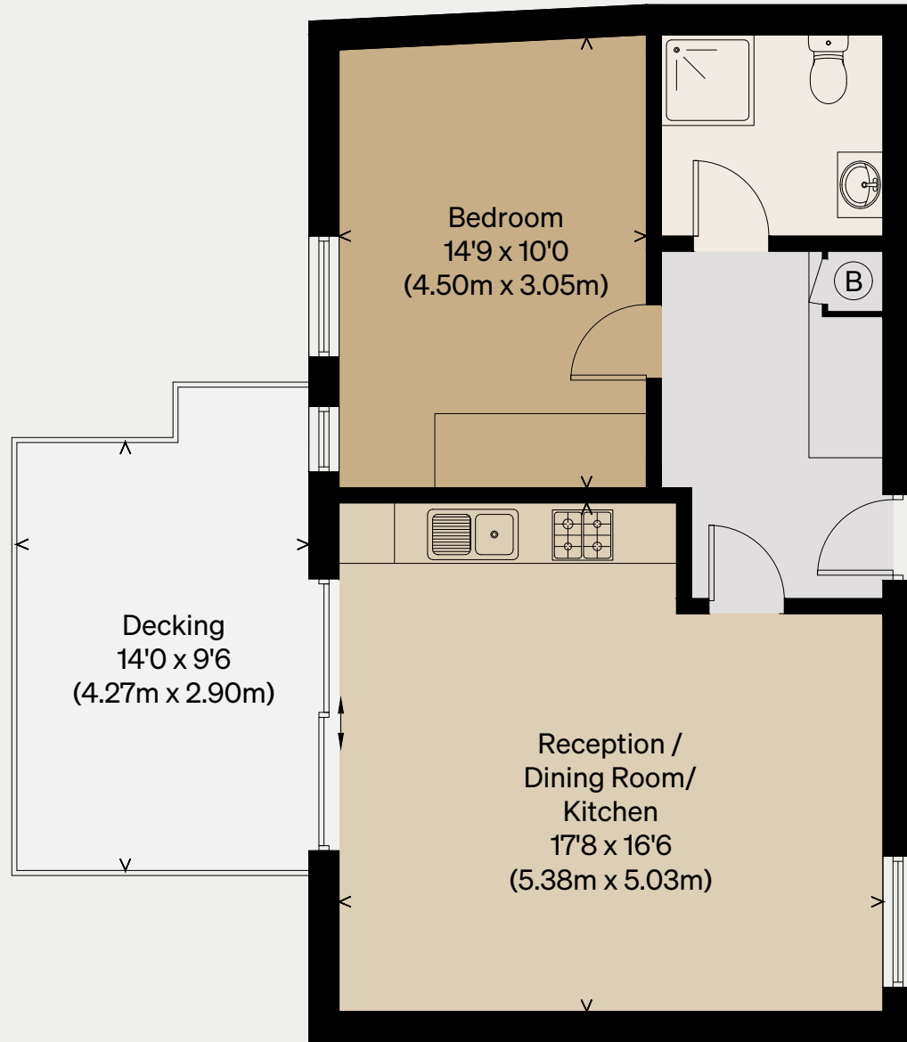
FIRST FLOOR
