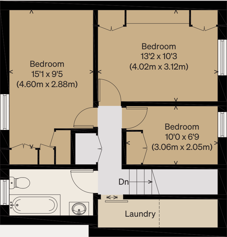
THIRD FLOOR
