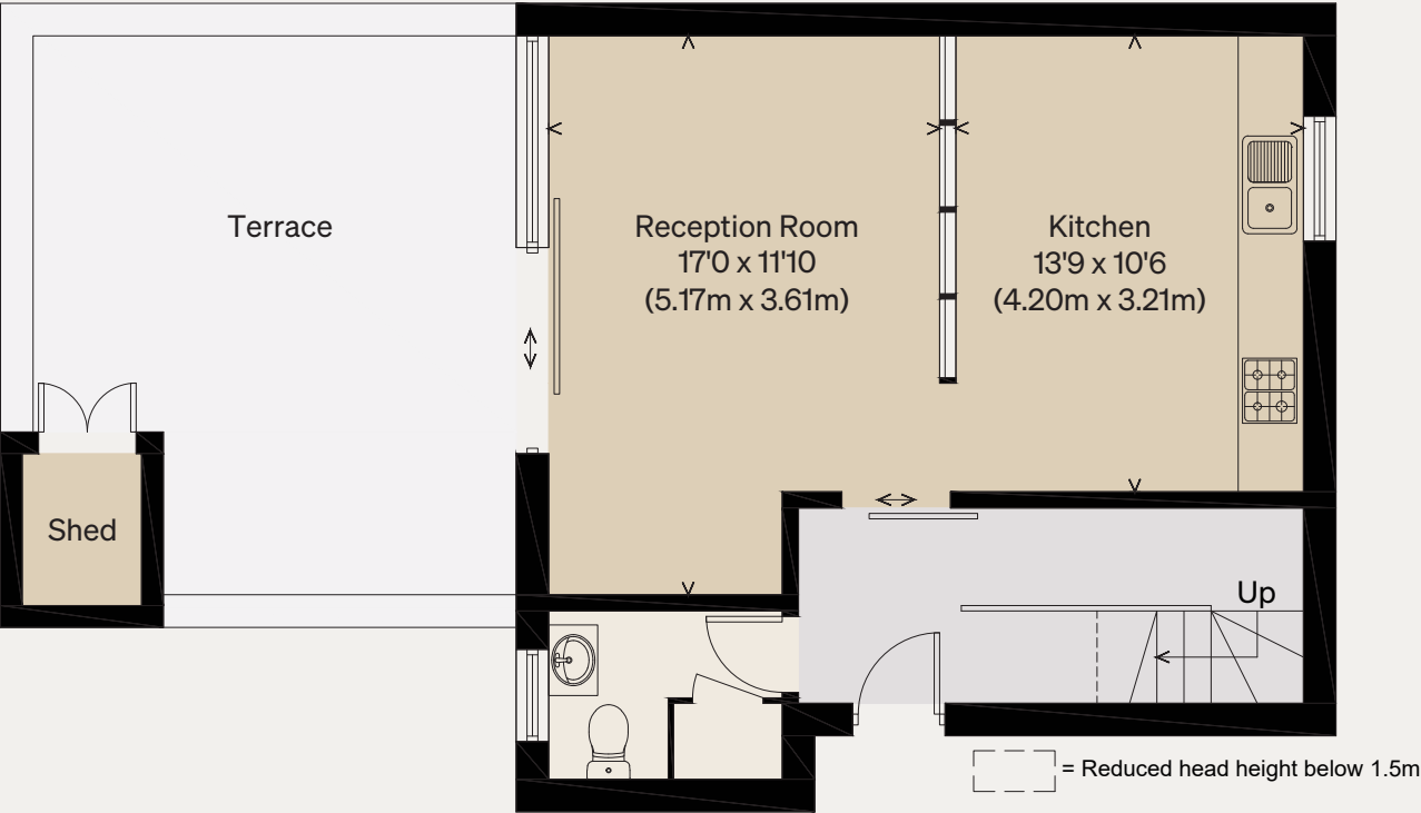
SECOND FLOOR
