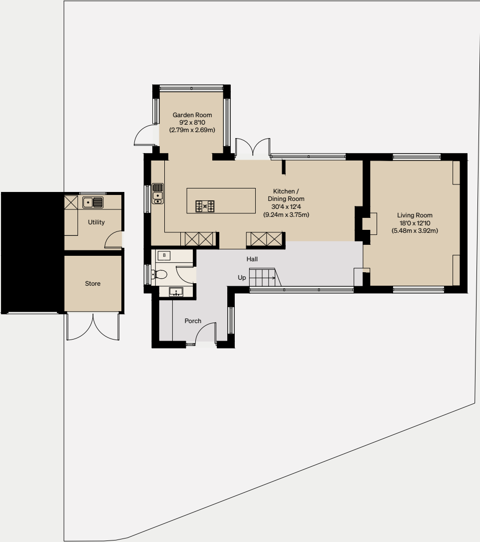
GROUND FLOOR
