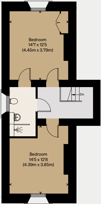
SECOND FLOOR
