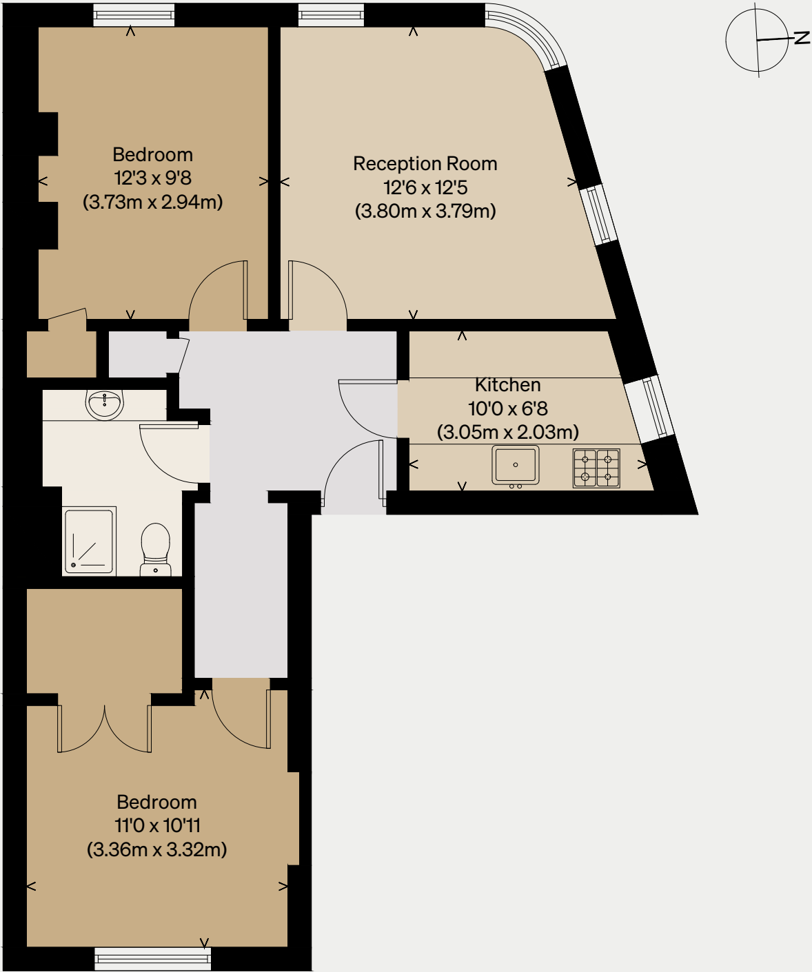
FIRST FLOOR
