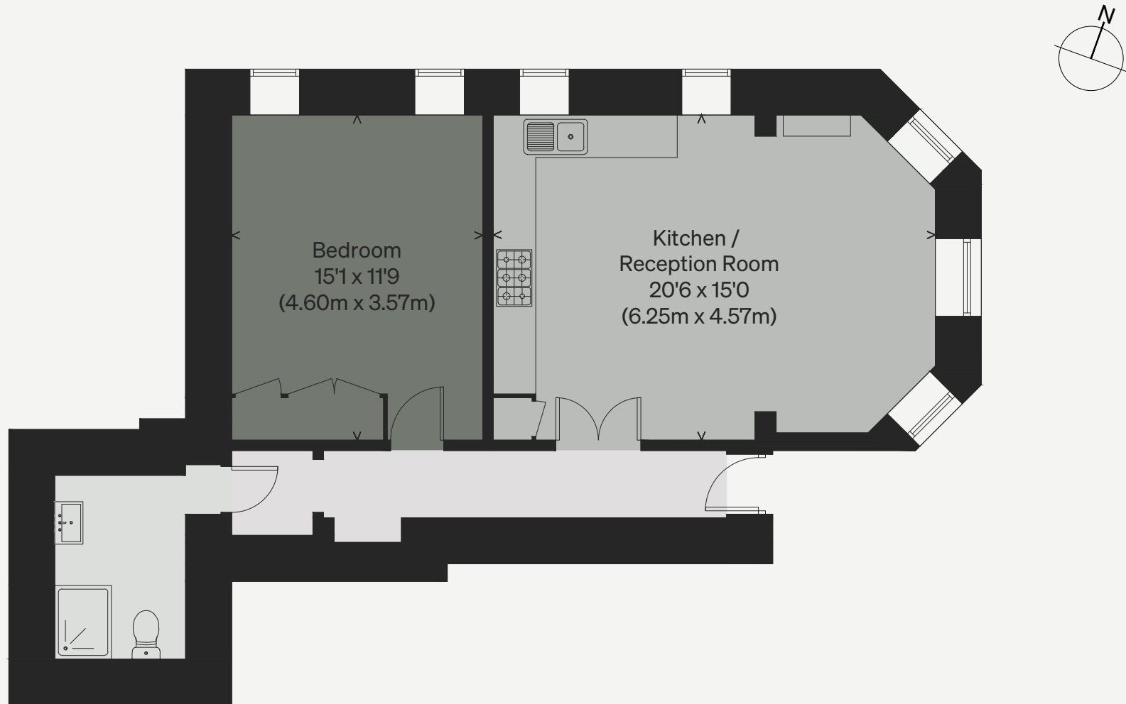
GROUND FLOOR
