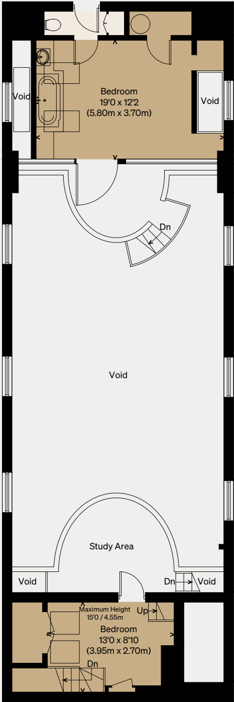
THIRD FLOOR
