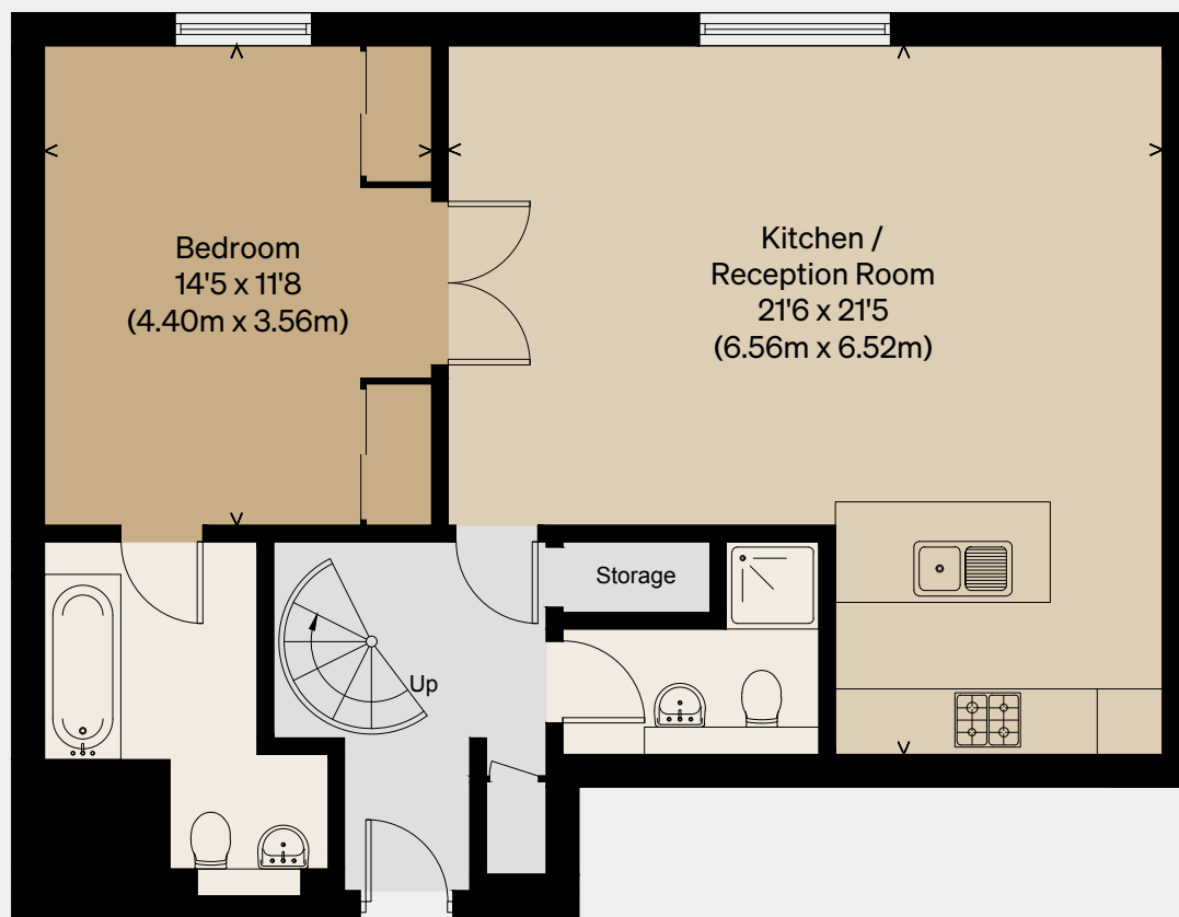
GROUND FLOOR
