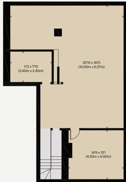
CELLAR FLOOR
