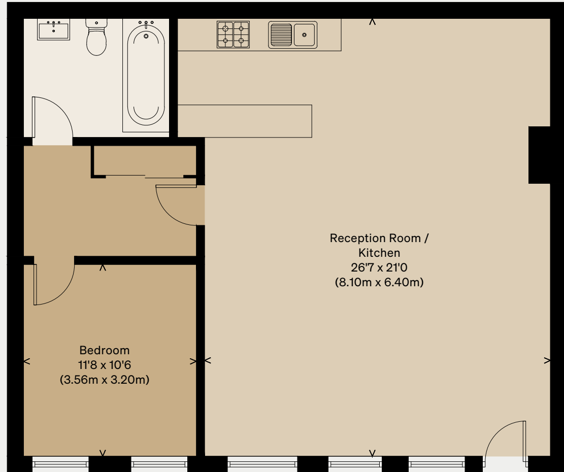
GROUND FLOOR
