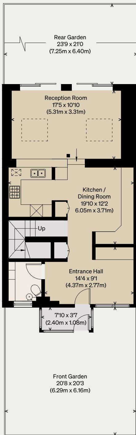
GROUND FLOOR
