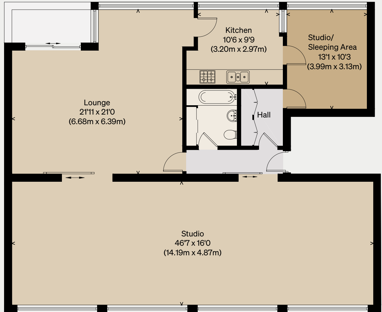
SECOND FLOOR
